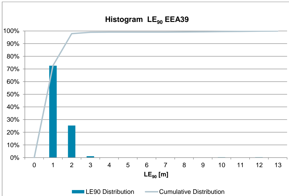
Figure 6: Histogram of the LE 90 distribution of the EEA39 area. The bins represent half open intervals, e.g. bin 2 includes all 2 \leq LE_{90} < 3 values.
