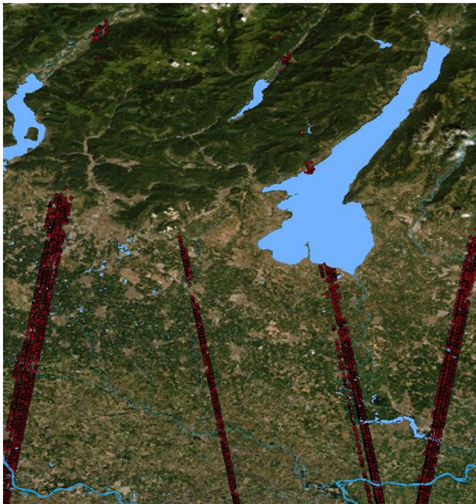
Figure 2: Image of filtered ICESat data (red points) – Lake Garda Northern Italy (Source: Esri World Imagery Basemap)
