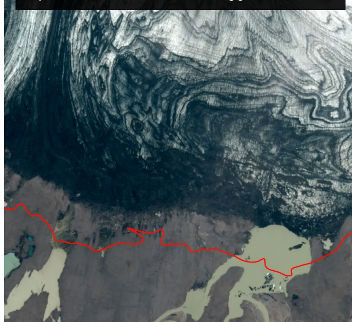
Copernicus Sentinel data 2025: Retreating glacier in Iceland
